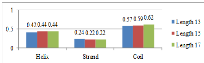
Figure 2. Accuracy of each Local Protein Structure based on Secondary Structural State
