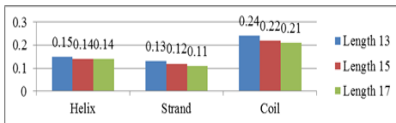
Figure 4. False Positive Rate of each Local Protein Structure based on Secondary Structural State
