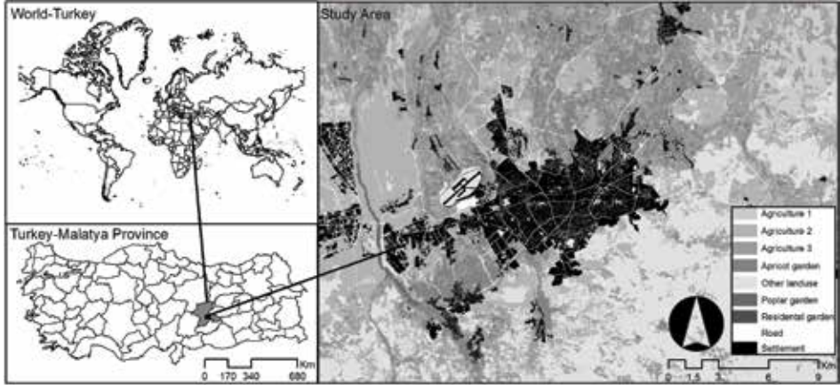
Fig. 2. Location of Malatya province and study area
