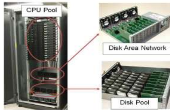
Figure 3: Actual Fujitsu Server Hardware Prototype.
